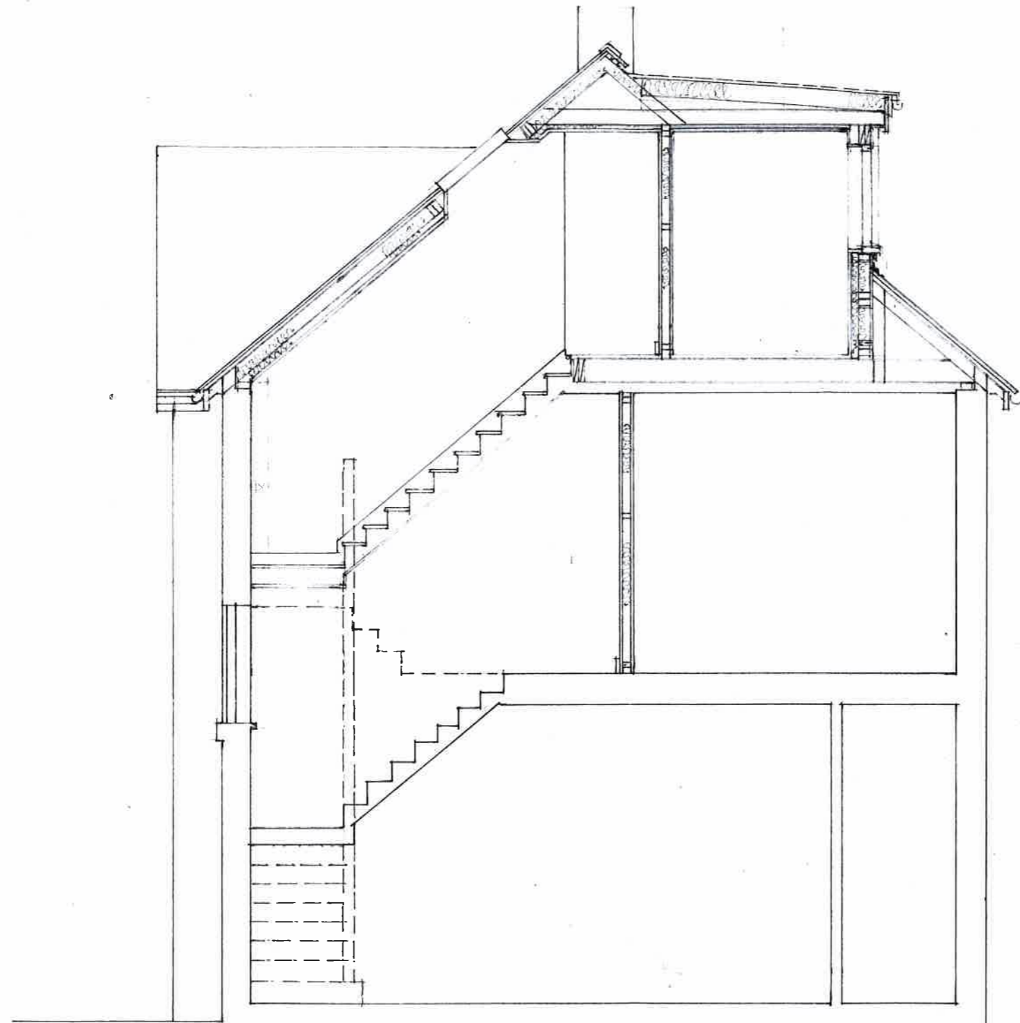
SECTION E-E
